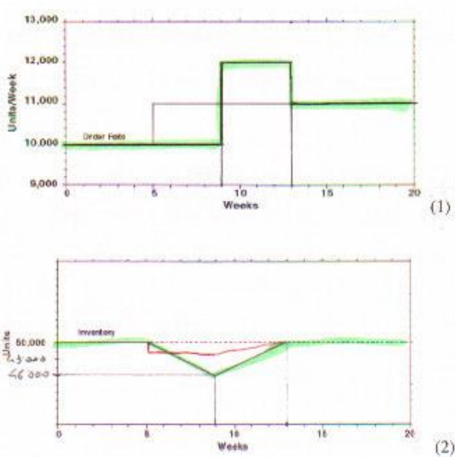
Figure 4.4.1. The Manufacturing test case (MC4), adapted from Sweeny and Sterman (2000).
