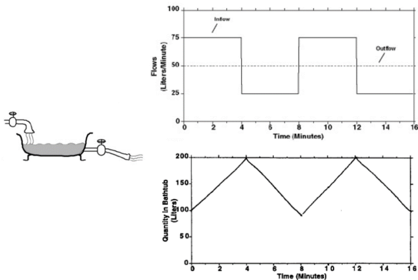
Figure 4.1.1. The Bathtub Dynamics test case (BT1), adapted from Sweeny and Sterman (2000).
