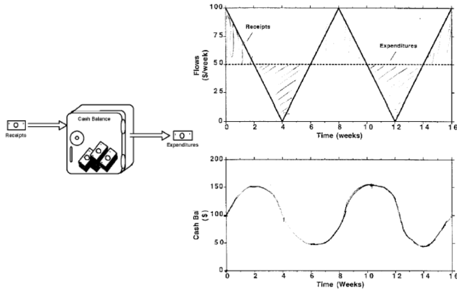
Figure 4.2.1. The Cashflow test case (CF2), adapted from Sweeny and Sterman (2000).
